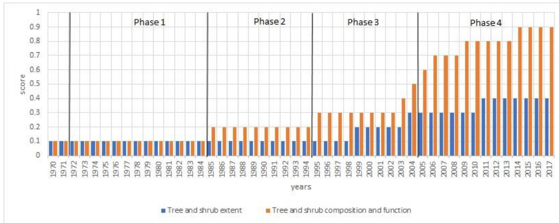
Figure 4. Status of trees and shrubs for production and to maintain ecological health of the property and watershed over time at Jillamatong
