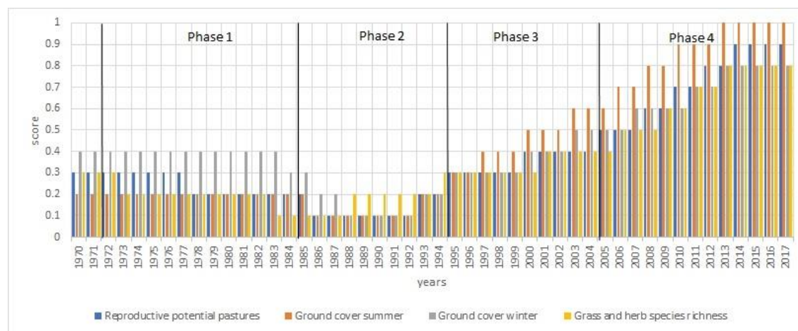
Figure 3. Status of ground layer vegetation for production and to maintain ecological health over time at Jillamatong
