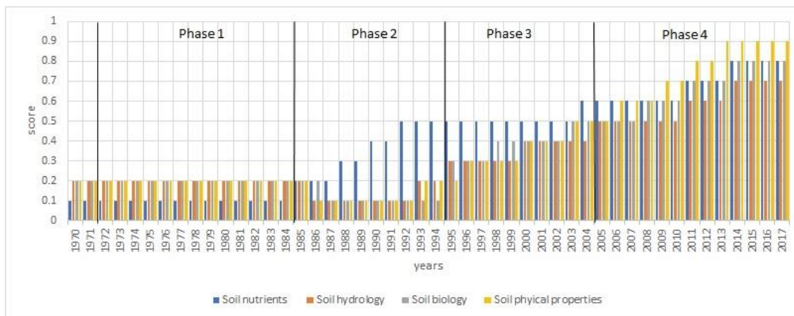
Figure 2. Status of soil indicators over time at Jillamatong.
